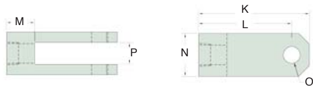
Clevis Dimensions
