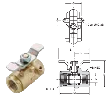
Tee Handle, Female Pipe Ends, Panel Mount V502P-X-04
