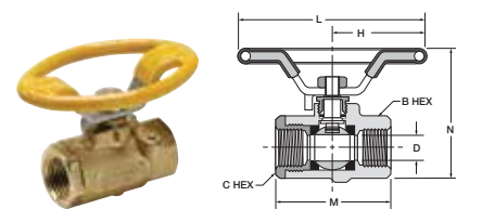
Oval Handle, Female Pipe Ends, Panel Mount V502P-X-21
